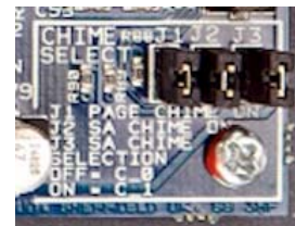
Jumpers for Chime Selection J1 – Voice Page Chime (on/off) J2 – Message Chime (on/off) J3 – Different Chimes for Voice & Message
